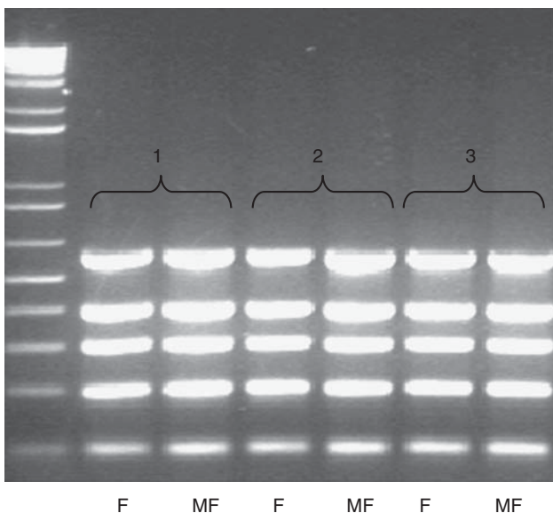
FIGURE 2. Multiplex PCR amplification for 5 different PCR sizes of products ranging from 100 to 600 bp for 3 paired frozen (F) and methanol-fixed paraffin-embedded (MF) tumors. PCR indicates polymerase chain reaction.
